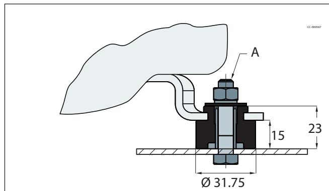
Figure: Silent bloc
