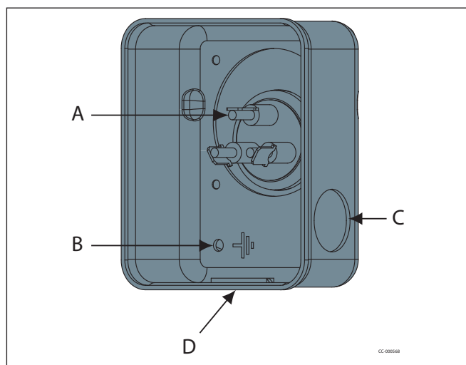
Figure: Terminal box for model (1)
