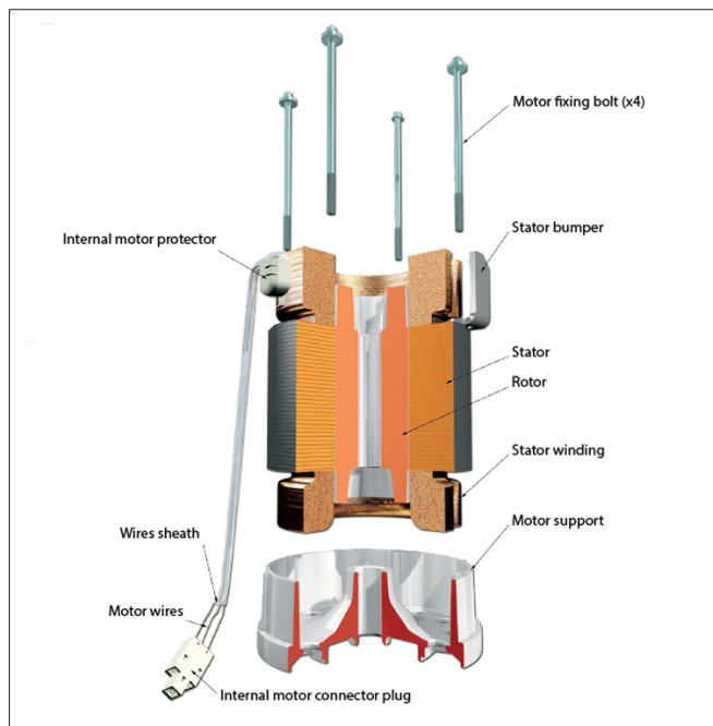
Figure: Motor
