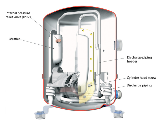
Figure: Discharge piping
