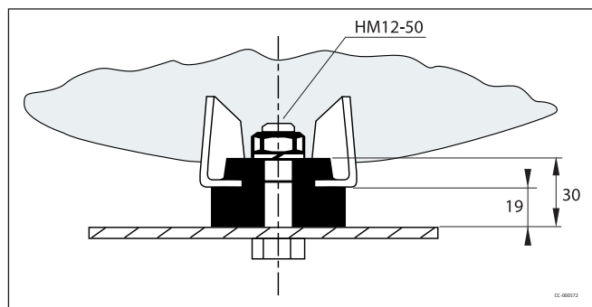
Figure: Silent bloc
