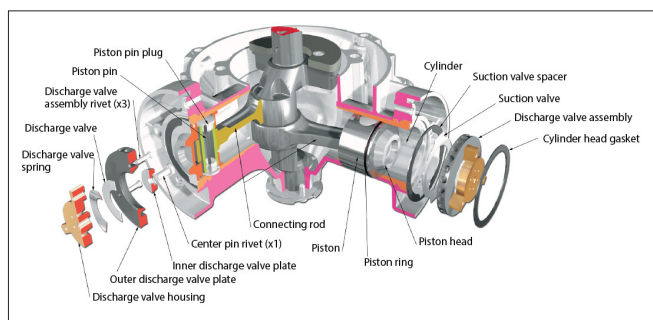
Figure: Compression sets assembly
