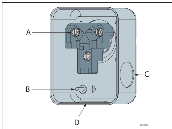
Figure: Terminal box for model (2)
